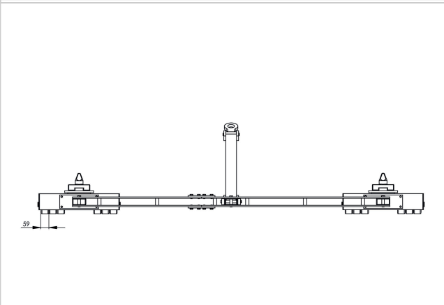
JTLB 30 G TL | Art.No. 12.302.140-TL | Frontansicht | Front view
