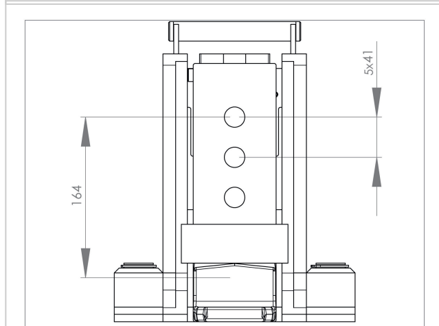
JH 10 G plus EX | Art.No. 11 610 106-G | Frontansicht | Front view
