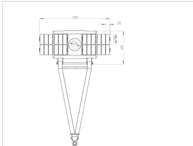
JLB 60 H | Art.No. 09 600 206-H Professional | Draufsicht | Top view
