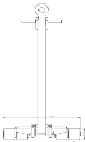
JLB 6 K | Art.No. 07 061 085-V | Frontansicht | Front view
